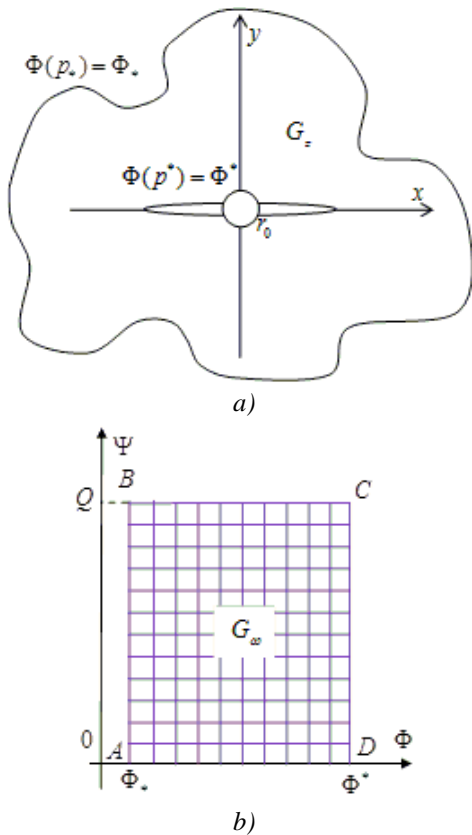
Figure 1 – Schematic layout of reservoir with hydraulic fracture (a) and correspondent complex potential area (b)
